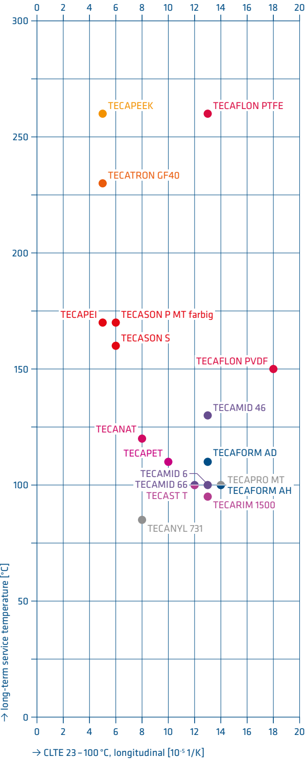
Coefficient of linear thermal expansion versus long-term service temperature
